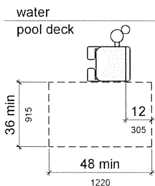
Figure 1009.2.3 Clear Deck Space at Pool Lifts
