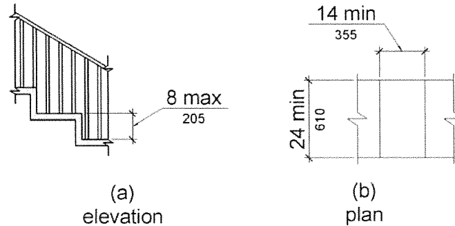
Figure 1008.3.2 Transfer Steps
