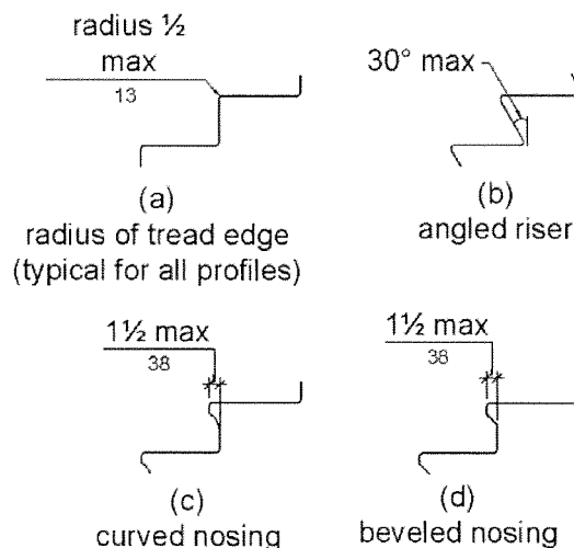
Figure 504.5 Stair Nosings
