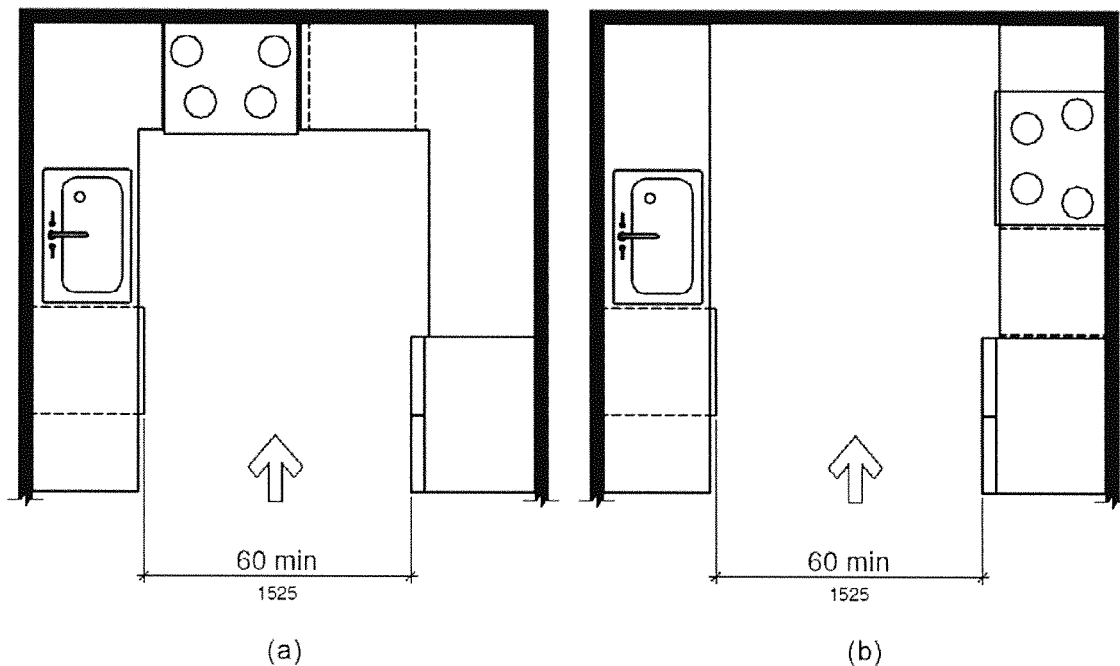
Figure 804.2.2 U-Shaped Kitchens
