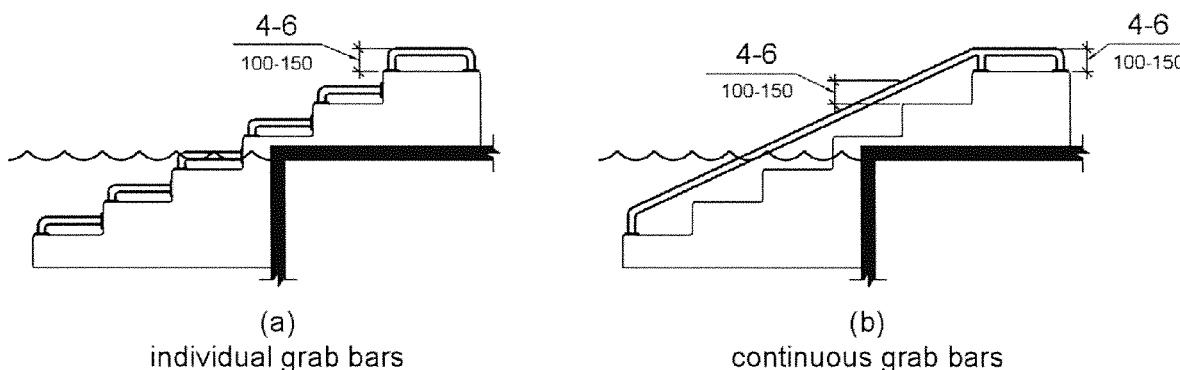
Figure 1009.5.7 Grab Bars
