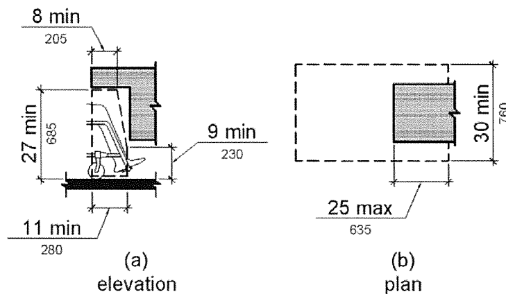
Figure 306.3 Knee Clearance
