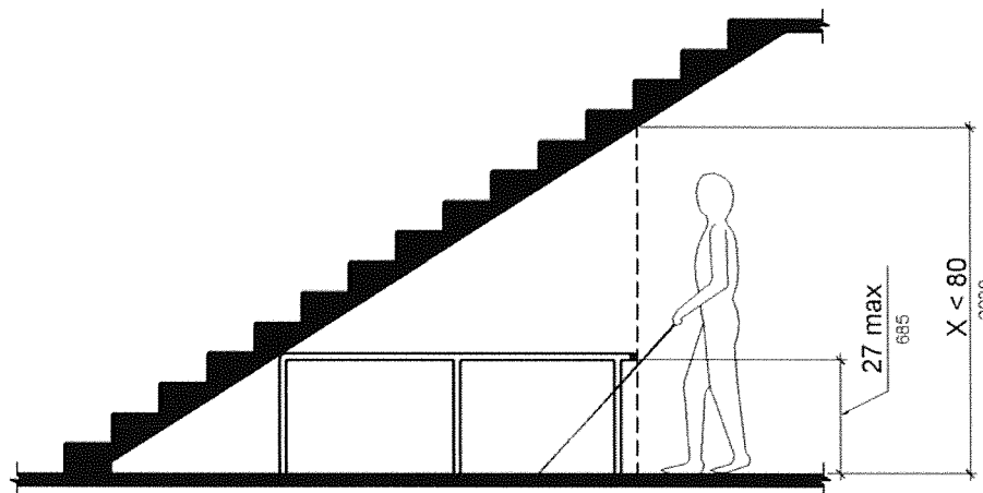
Figure 307.4 Vertical Clearance
