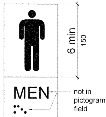
Figure 703.6.1 Pictogram Field
