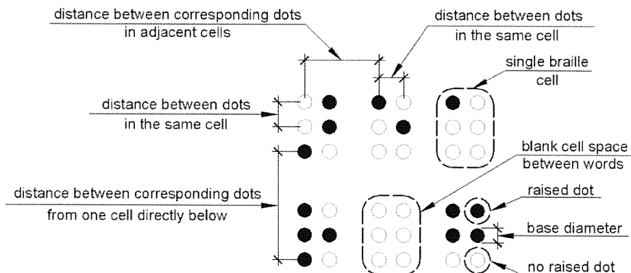
Figure 703.3.1 Braille Measurement
