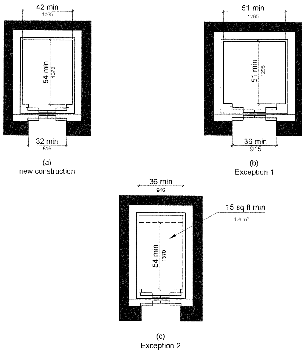
Figure 408.4.1 Limited-Use/Limited-Application (LULA) Elevator Car Dimensions
