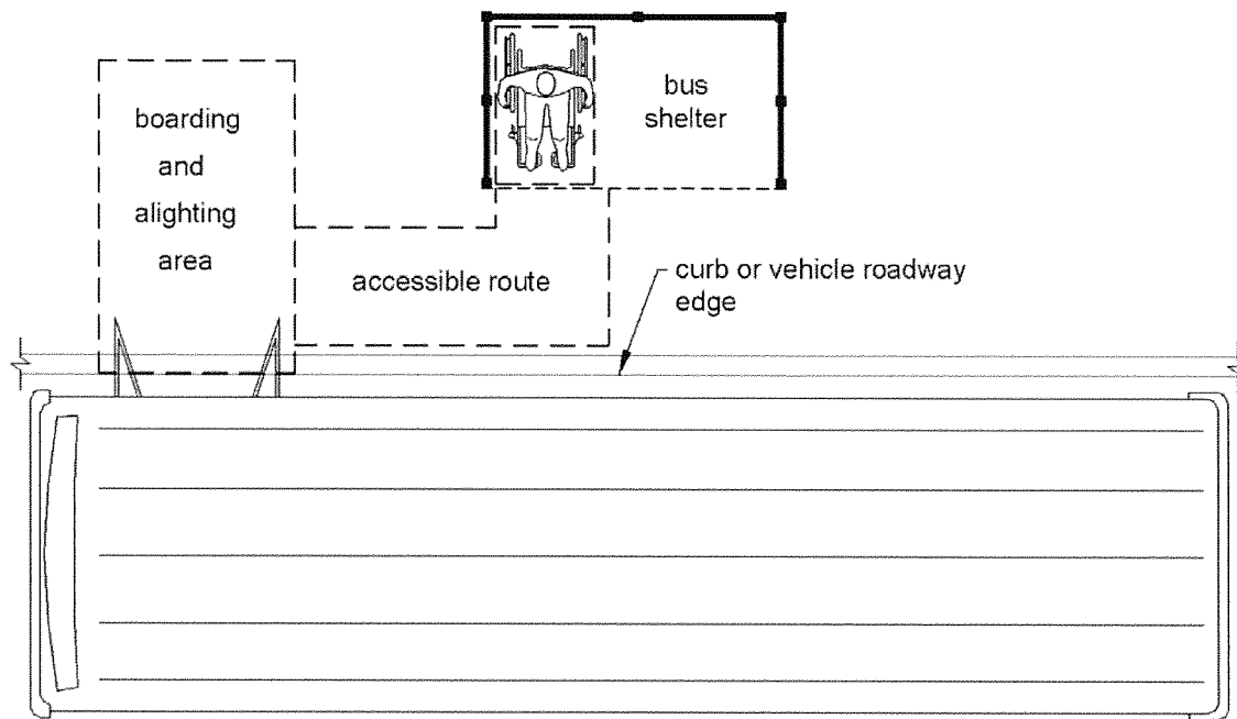
Figure 810.3 Bus Shelters
