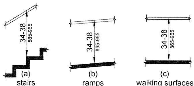
Figure 505.4 Handrail Height
