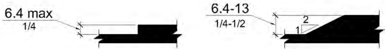
Figure R302.7.2 Vertical Surface Discontinuities
