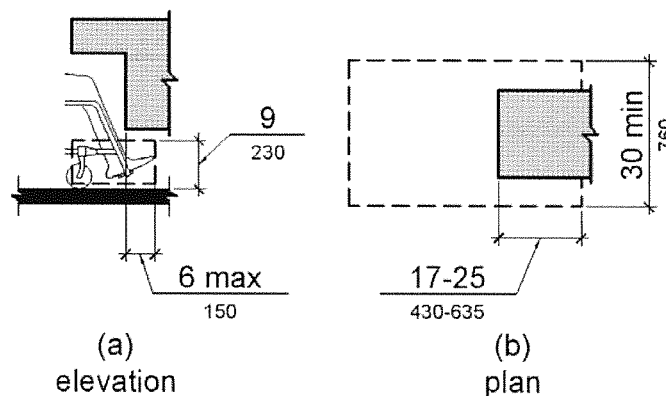
Figure 306.2 Toe Clearance
