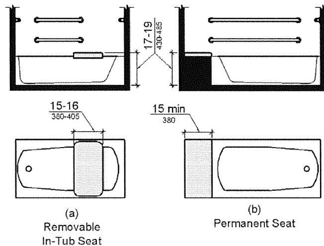
Figure 610.2 Bathtub Seats
