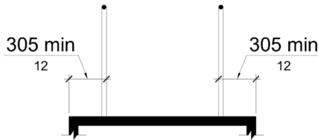
Figure R407.9.1 Extended Ramp Surface
