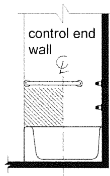
Figure 607.5 Bathtub Control Location
